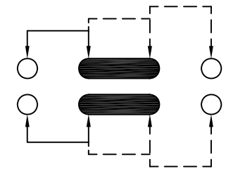
SCHEMATIC (NON-SHORTING)
